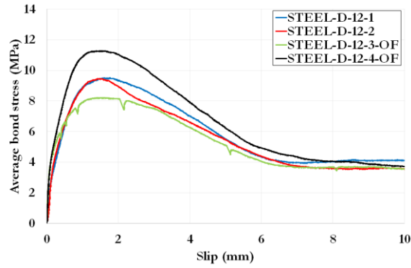
Fig 7. Bond-slip curves for RC specimens with STEEL-D-12 rebars
