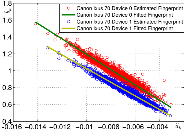
Figure 4: Illustration of linear relationship between the parameters (\bar{a}_k, \bar{b}_k) which are used as fingerprint for camera device identification; the results have been obtained following the process described in Section IIb fitted by using Least Square algorithm (LS).
