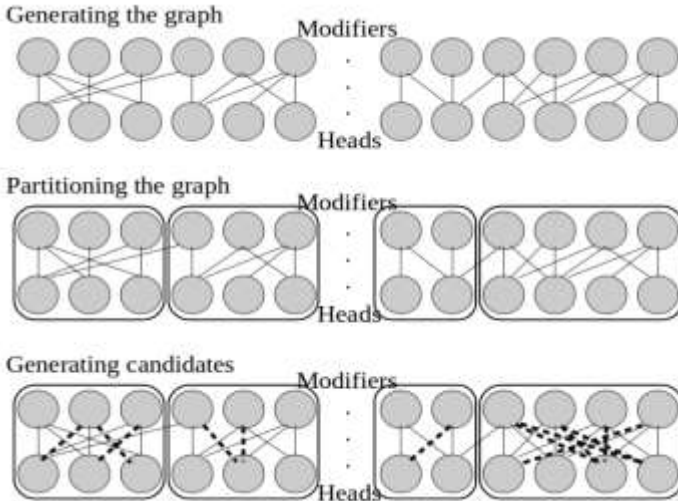
Figure 9. Generating extended head-modifier pairs
