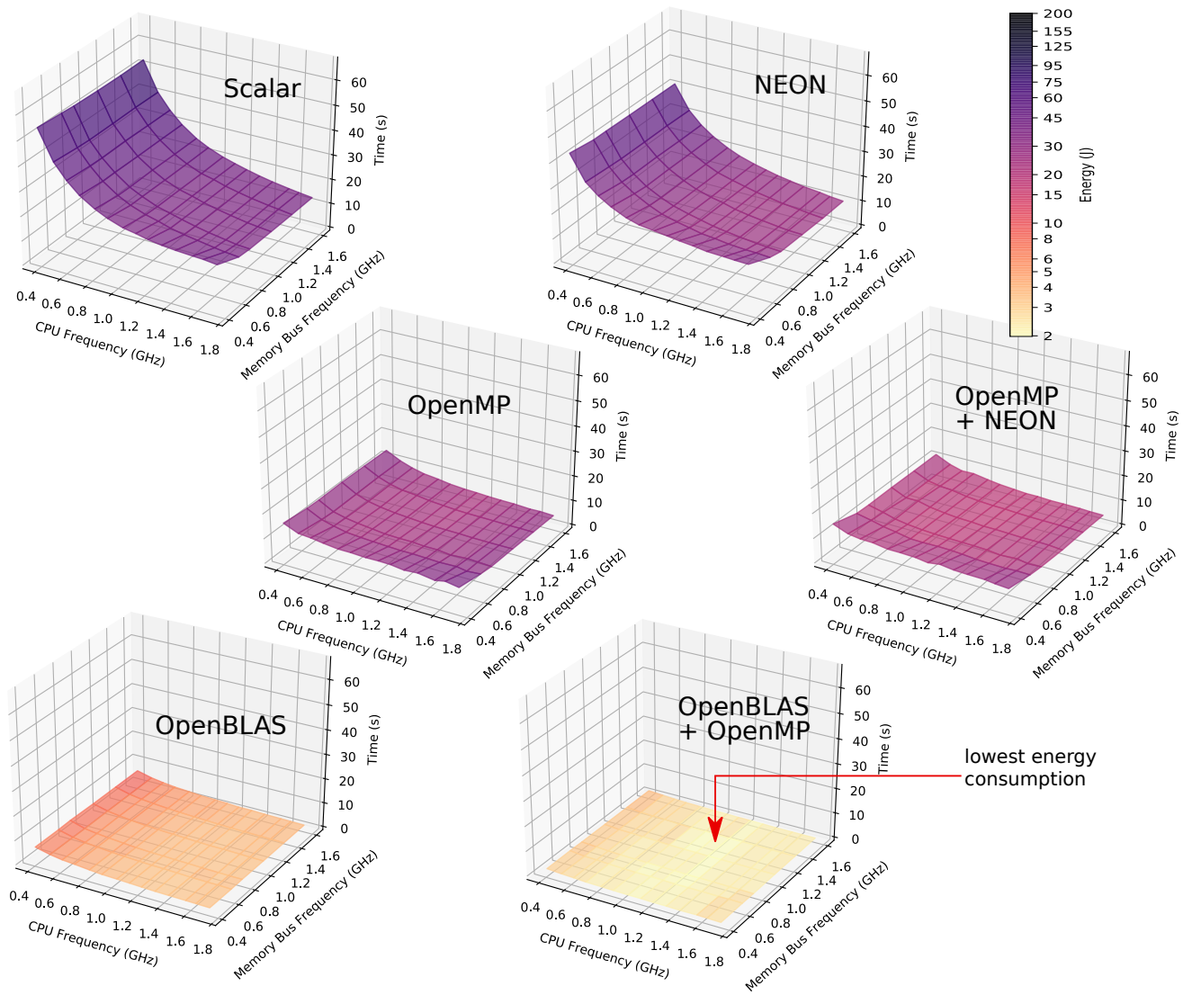
Fig. 9: Performance of the matrix multiplication implementations depending on the CPU and memory bus frequencies. The color represents the energy.
