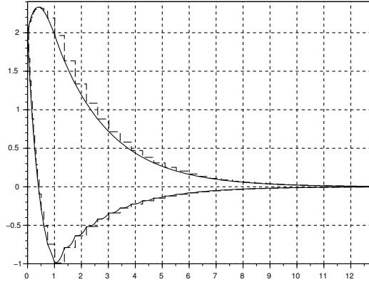
Fig. 2: Gain synthesis: Trajectory of the system using K = [0.8, -5.3] , plain x(t) state of the system, dashed sampled value z(t) .
