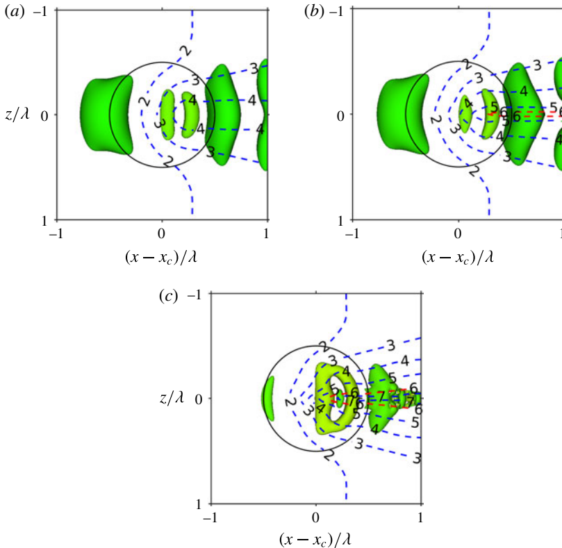
FIGURE 18. (Colour online) Comparison of laminar–turbulent transition onsets for different h in a local domain around indentation. The parameter \lambda = 81 mm. (a) h = 1.620 mm; (b) h = 1.895 mm; (c) h = 2.170 mm. The iso-surfaces are generated by pressure fields. The red dashed lines indicate the contour lines with the transition criteria N -factor 6. The solid circles indicate the indentation boundaries r = \lambda/2 .
