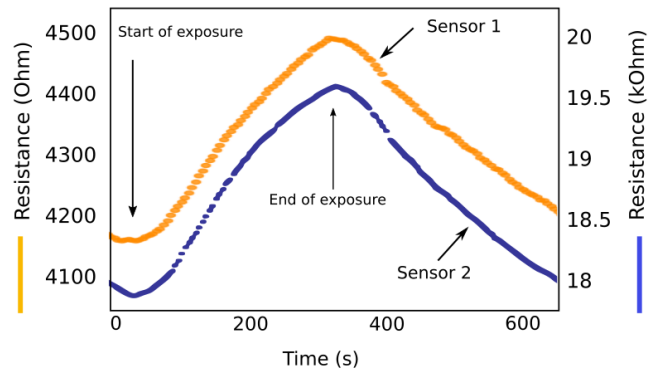
Fig. 5. Resistance variation of sensors 1 and 2 to 1.5 ppm of ammonia and human breath composition.
