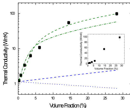
FIG. 3. Computed (black points), EMA model (with and without R_K blue dot line and blue dash line respectively) and EMA with percolation (dash-dot for normal set of parameters and dash for 2VF) TC as a function of volume fraction. In the inset the MD results are displaced to show clearly the threshold of percolation.
