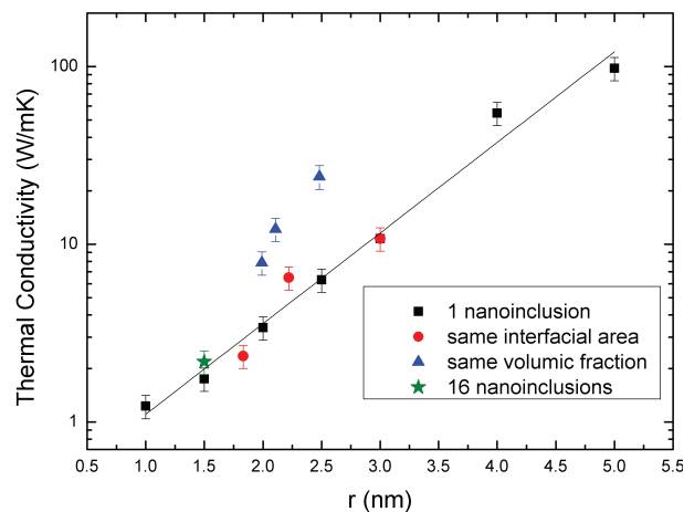
FIG. 8. TC for all studied systems as a function of the radii of the nanoinclusions.
