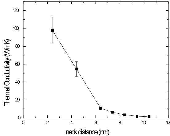
FIG. 4. TC as a function of the amorphous neck distance between two nanoinclusions
