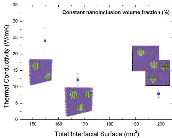
FIG. 7. (Color online) TC as a function of the total interfacial area upon increasing the number of nanoinclusions at constant volume fraction (b). The facets of the insets are different each time to visualise in a more efficient way the spatial distribution of the nanoinclusions.
