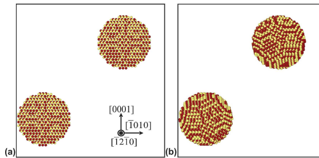
FIG. 5. Two modeled systems with the same volume fraction of two GaN nanoinclusions inside an amorphous silica matrix: (a) the two nanoinclusions have the same relative orientation, (b) the two nanoinclusions have been rotated by 60^\circ in both x and y directions.
