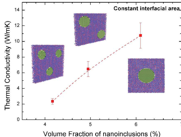
FIG. 6. TC as a function of the Volume Fraction upon increasing the number of nanoinclusions, but for the same total interfacial area.
