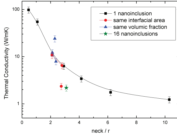
FIG. 9. TC for all studied systems as a function of the ratio of the distance between two neighboring nano-inclusions (neck) divided by the radius of the nano-inclusions.
