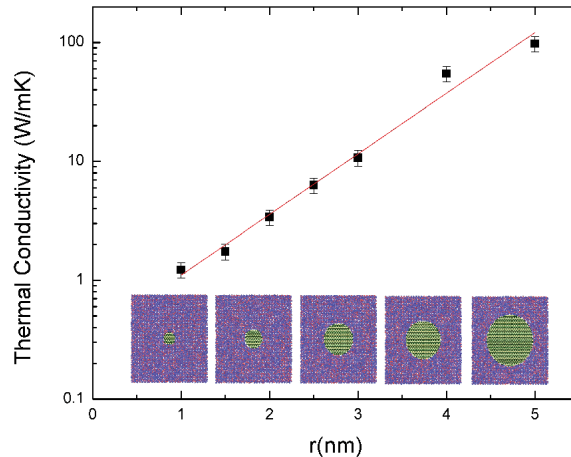
FIG. 2. Computed TC with MD as a function of nanoinclusion radius
