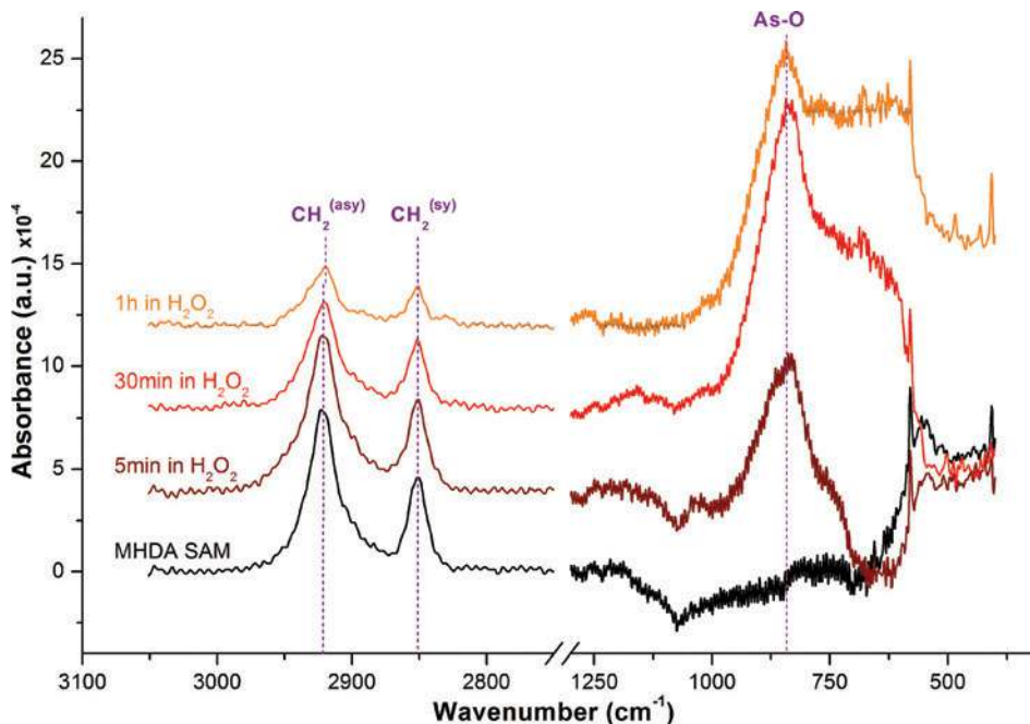
FIG. 2. Infrared spectra of MHDA SAM coated GaAs (100) samples immersed in hydrogen peroxide ( \text{H}_2\text{O}_2 ) for various soaking time.
