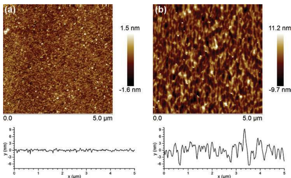
FIG. 5. Examples of AFM images of GaAs (001) surface originally functionalized with MHDA (a), and refunctionalized with MHDA after 2 min etching in 3 \text{NH}_4\text{OH}:\text{H}_2\text{O}_2:\text{H}_2\text{O} .
