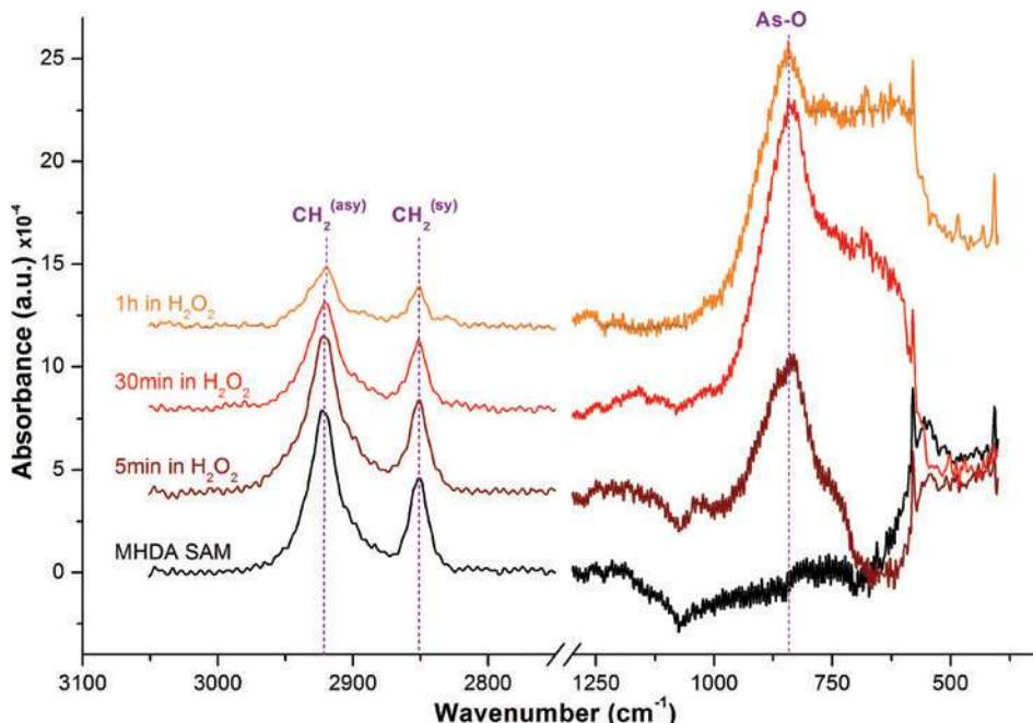
FIG. 2. Infrared spectra of MHTA SAM coated GaAs (100) samples immersed in hydrogen peroxide ( \text{H}_2\text{O}_2 ) for various soaking time.
