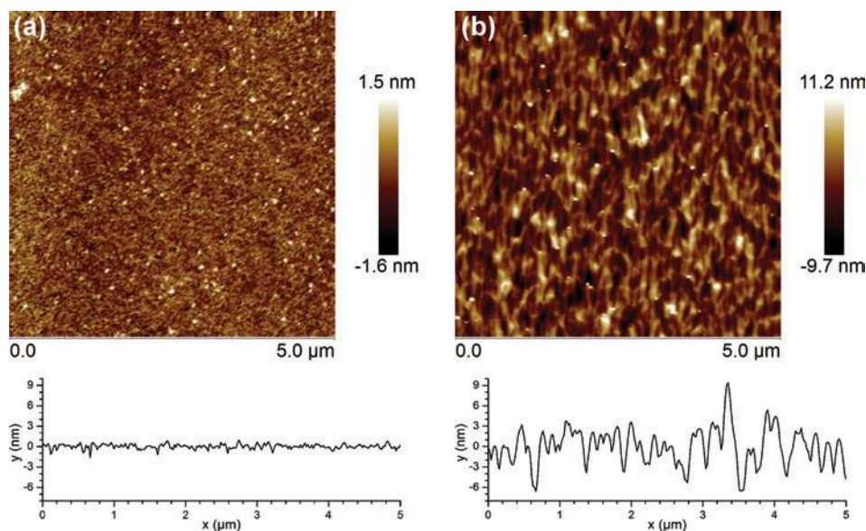
Fig. 5. Examples of AFM images of GaAs (001) surface originally functionalized with MHDA (a), and refunctionalized with MHDA after 2 min etching in 3\text{ NH}_4\text{OH}:1\text{ H}_2\text{O}_2:100\text{ H}_2\text{O} .
