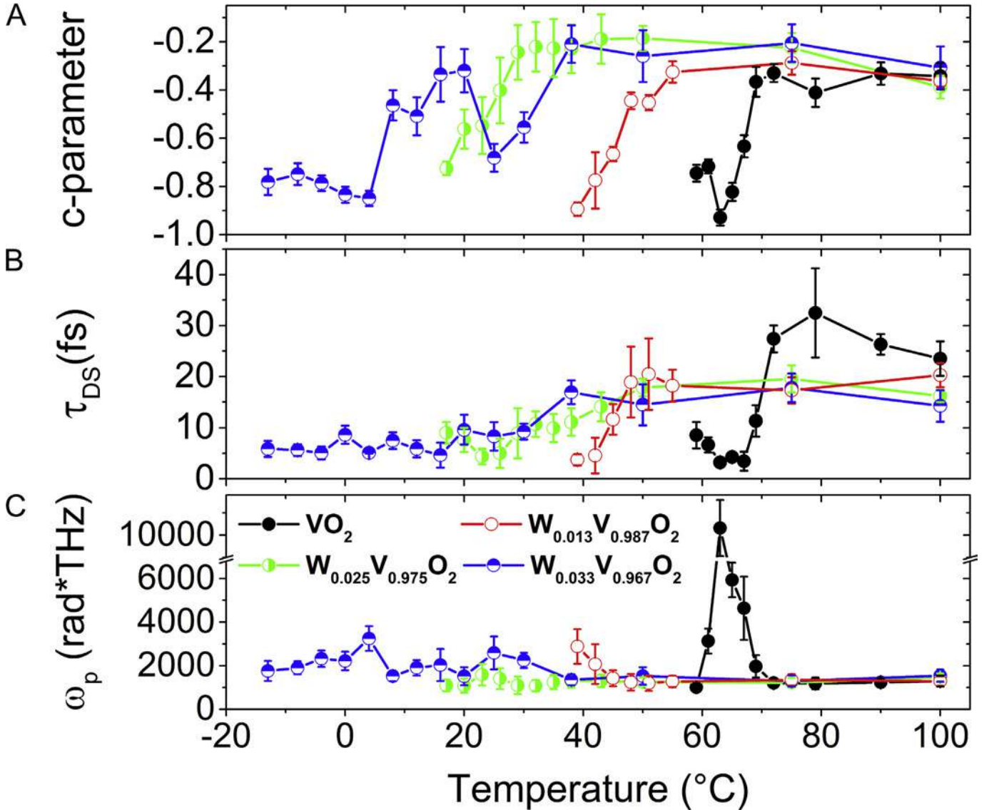
Fig. 7. Temperature dependence of the \text{W}_x\text{V}_{1-x}\text{O}_2 thin films Drude-Smith parameters (A) c parameter, (B) scattering time ( \tau_{DS} ) and (C) plasma frequency ( \omega_p ).
