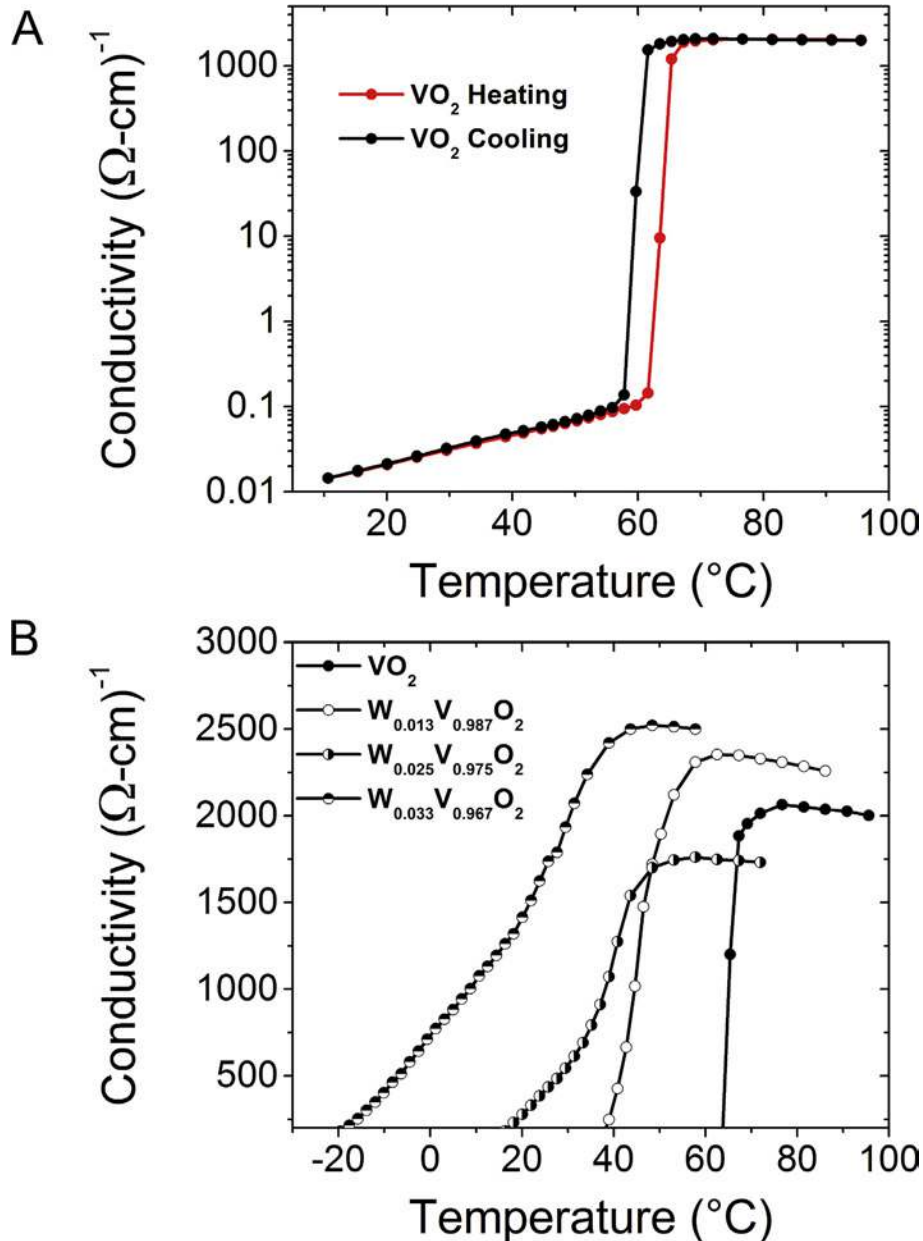
Fig. 3. Temperature-dependent DC conductivity of (A) the VO_2 thin film on Al_2O_3 (1T02) for heating (red curve) and cooling (black curve) segments and (B) W_xV_{1-x}O_2 thin films on Al_2O_3 (1T02) using a standard four point geometry. (For interpretation of the references to colour in this figure legend, the reader is referred to the web version of this article.)
