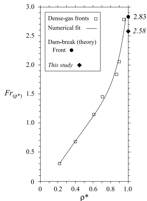
Figure 12. Froude number Fr_{(\rho^*)} = U_f/(gh_f)^{1/2} as a function of \rho^* = [(\rho_{\text{dense}} - \rho_{\text{light}})/(\rho_{\text{dense}} + \rho_{\text{light}})]^{1/2} for fluid gravity currents and our experimental flows with particles of group A propagating in an infinite ambient medium; see text for details. Modified after Gröbelbauer et al. [1993].
