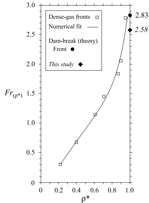
Figure 12. Froude number Fr_{(\rho^*)} = U_f/(gh_f)^{1/2} as a function of \rho^* = [(\rho_{dense} - \rho_{light})/(\rho_{dense} + \rho_{light})]^{1/2} for fluid gravity currents and our experimental flows with particles of group A propagating in an infinite ambient medium; see text for details. Modified after Gröbelbauer et al. [1993].
