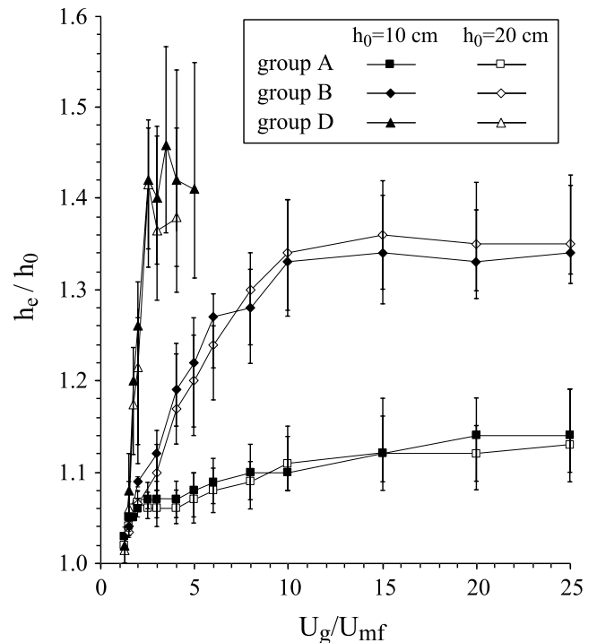
Figure 3. Expansion of the bed in the reservoir as a function of the degree of fluidization ( U_g/U_{mf} ), h_e and h_0 are the height of the expanded and nonexpanded beds, respectively. Mean values and range of bed height variations are shown for bubbling beds. Bubbles form at U_g/U_{mf} = 1 for groups B and D particles and at U_g/U_{mf} \approx 2 for group A particles. Experiments at U_g/U_{mf} > 2.5 were not studied in detail for group D particles.
