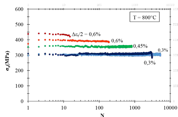
Fig.3. Stress amplitude versus number of cycles of IRIS alloy at 800°C.
