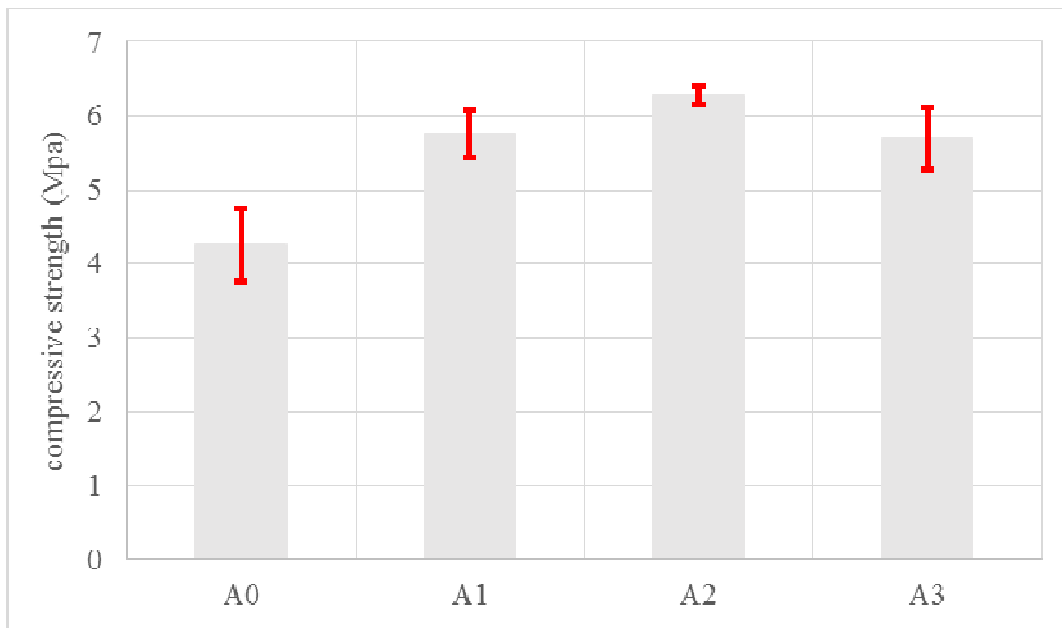
Figure-8: Compressive Strength - Influence of the length of the Kenaf fiber.
