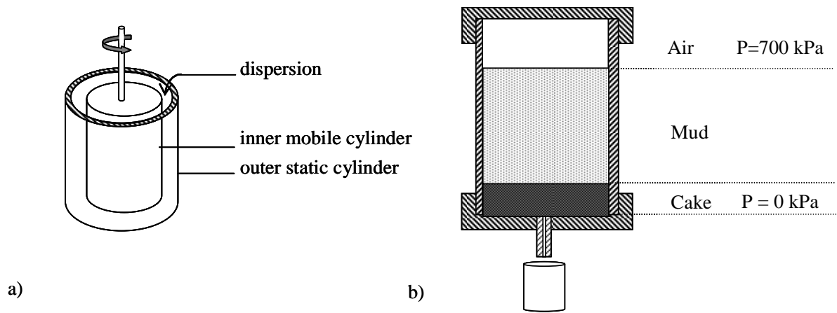
Figure 1. Schematic of the rheometer geometry (a) and the filter press cell (b).
