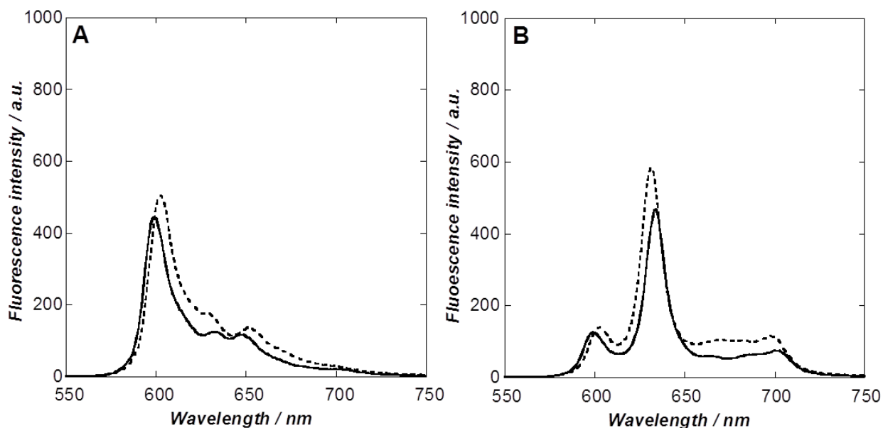
Figure 2. Fluorescence emission spectra (550-750 nm) of PpIX (1.25 μM) + Hy (1.25 μM) dissolved in DMSO ( dotted line ) and PpIX-Hy-loaded LNC25 ( continuous line ) in water at 2.5 μM. The emission spectra are recorded using an excitation wavelength \lambda_{\text{ex}}=330 nm ( A ) and 410 nm ( B ).
