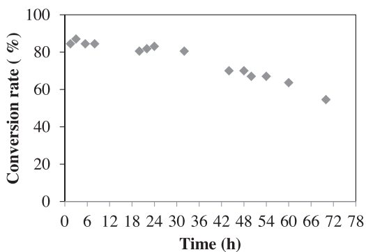
Fig. 8. Conversion in the CPR for a 3 day operation. Reaction conditions: 3 \text{ g L}^{-1} of enzyme, n\text{-BuOH/acid} ratio of 3, 2.5 \text{ mL min}^{-1} flow rate and 800 \text{ rpm} rotation speed. CPR is operated at controlled room temperature ( 22^\circ\text{C} ).
