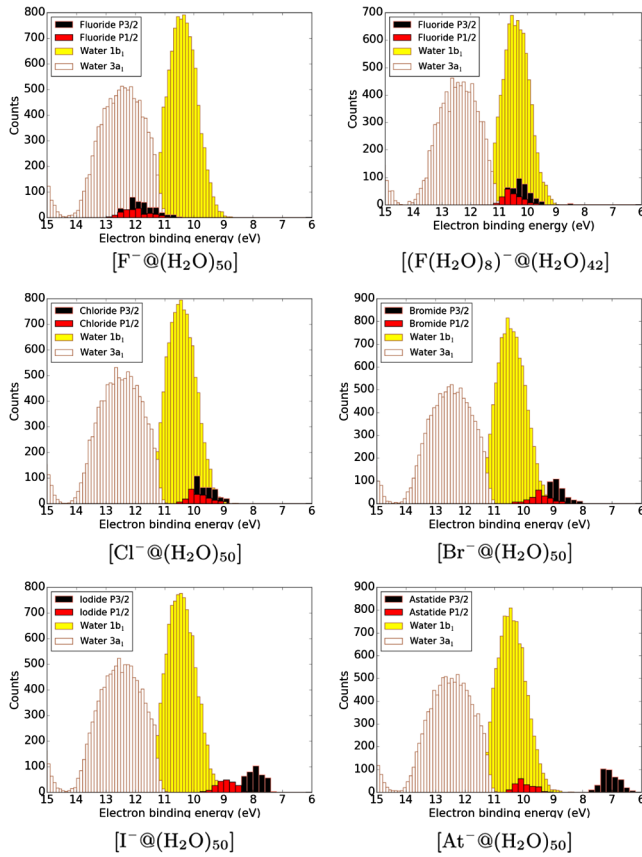
FIG. 2. Electron binding energies spectra for the [X^-@(\text{H}_2\text{O})_{50}] systems over the 100 snapshots. Halides BEs obtained with triple-zeta basis sets from DC EOM [except for [(\text{F}(\text{H}_2\text{O})_8)^-@(\text{H}_2\text{O})_{42}] obtained with DC SAOP] [68].
