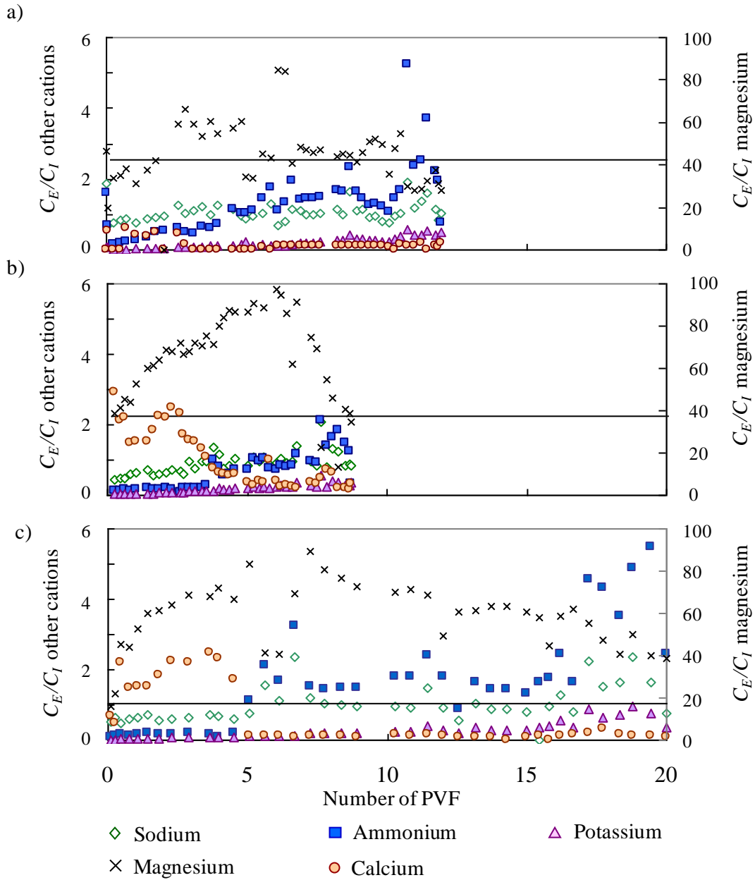
Fig. 7: Effluent-to-influent ratio of the cation concentrations ( C_E/C_I ) according to the number of PVF for oedopermeameter tests realised on: (a) LX1; (b) LX2; and (c) LX5 permeated by ML.
