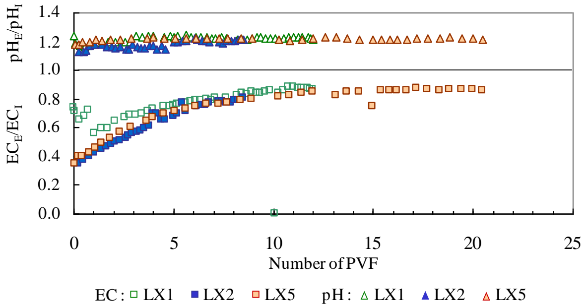
Fig. 6: Effluent-to-influent ratio of EC and pH during the oedopermeameter tests according to the number of PVF.
