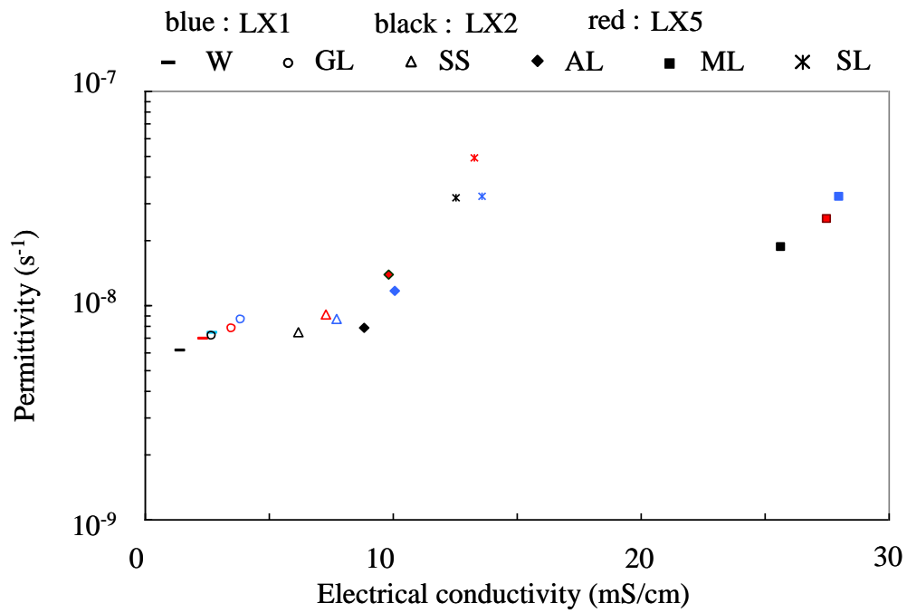
Fig. 2: Permittivities obtained with the filter press under a 700 kPa air pressure according to the electrical conductivity of the dispersion. SL and W points were performed by Rosin-Paumier et al. (2010b).
