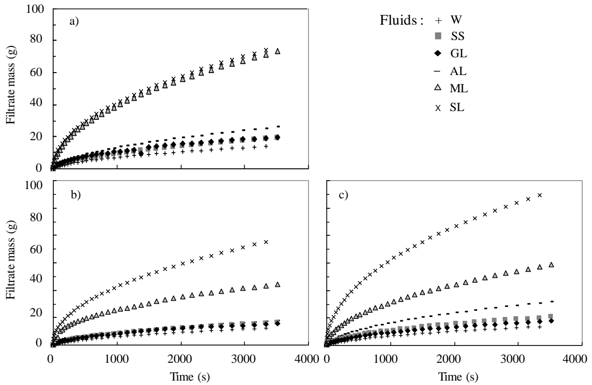
Fig. 1: Filtration curves for a) LX1; b) LX2 and c) LX5 dispersed in AL, SS, GL, ML (this study), osmosed water (W) and a synthetic leachate (SL) curves are from Rosin-Paumier et al. (2010b).
