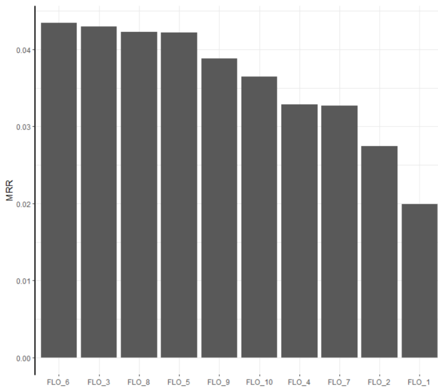
Fig. 2. MRR achieved by the 10 runs we submitted to the GeoLifeCLEF 2018 challenge
