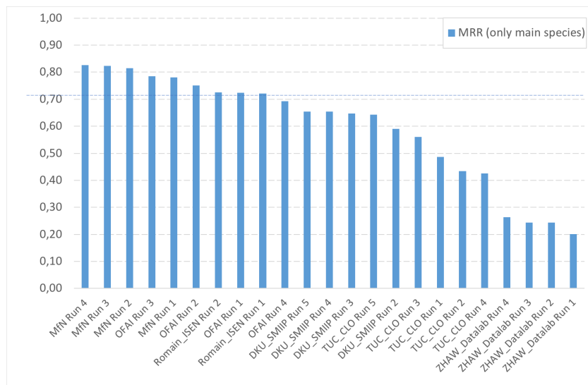
Fig. 3. BirdCLEF 2018 monophone identification results - Mean Reciprocal Rank. The blue dot line represents the last year's best system obtained by DYN I UTLN (Run 1) with a MRR of 0.714 [38].
