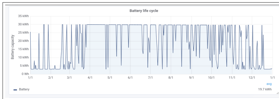
(b) Yearly battery usage, because of the long series of energy excess the battery is under used from April to October
