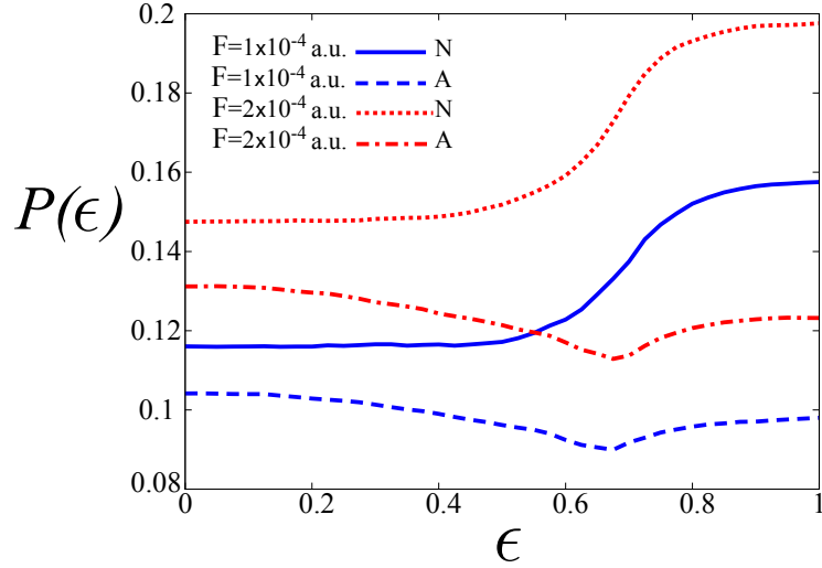
FIG. 14. Formation probabilities for the (small) laser intensities F = 1 \times 10^{-4} a.u. and F = 2 \times 10^{-4} a.u. calculated numerically (label N) and with the approximate expression (23) (label A). In all cases, the probabilities have been calculated for an initial ensemble of initial conditions with energy E_0 = 3 \times 10^{-9} a.u. The parameters of the pulse are T_{\text{ru}} = 15 ps, T_p = 70 ps and T_{\text{rd}} = 15 ps.
