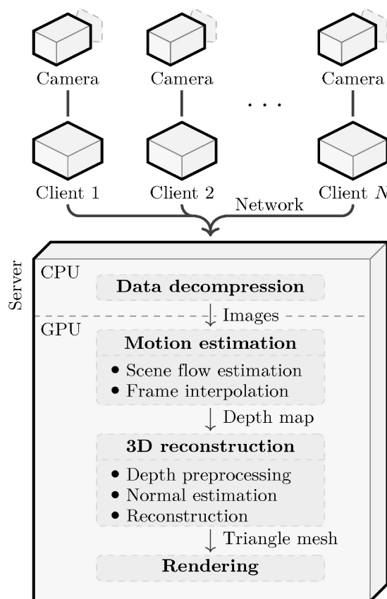
Fig. 1 FusionMLS pipeline.
