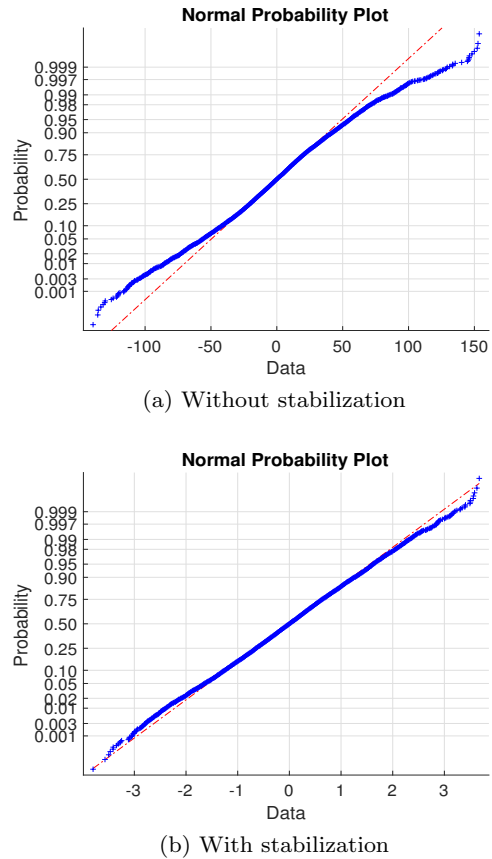
Fig. 2: Normal plot showing the distribution of the 3-dimensional wavelet coefficients d_{j,\mathbf{k}}^{l,m}(f_\varepsilon) , at the finest scale of the diagonal sub-band, with and without the stabilization step (“Liver” sequence).
