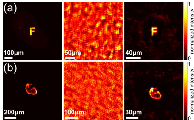
Fig. 11. A simple (a) and a more complex object (b), its scattered light after the diffuser (center row) and the reconstruction (right row). (a) 'F' pattern fabricated by direct laser writing process with organic dyes fluorescent structures in a clear polymer. (b) Drop casted orange beads.
