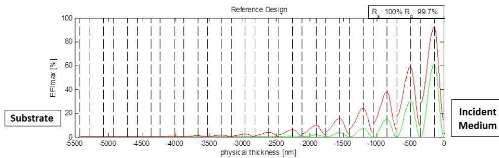
Fig. 1. Electric Field Intensity distribution for s (green) and p (red) polarization in a (HL)^{15}H stack where H is \text{HfO}_2 and L is \text{SiO}_2 . The incident medium, air, is located on the right of the stack and the substrate on the left. The electric field distribution is expressed as a percentage of the incident electric field intensity.
