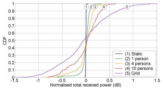
Fig. 2. Empirical CDF of the total received power.
