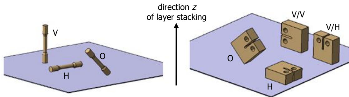
Figure 1: Orientations of the samples for tensile and toughness tests
