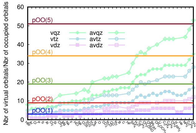
FIGURE 1. Number of virtual orbitals in terms of multiples of the number of occupied orbitals for the atoms and molecules considered in this paper. In filled symbols are the cc-pVXZ basis sets, denoted “vdz”, “vtz” and “vqz”, and in shallow symbols are the aug-cc-pVXZ, denoted “avdz”, “avtz” and “avqz”. The sets of pOOs up to a given order each yield a constant number of virtual orbitals in terms of multiples of the number of occupied orbitals, shown by the horizontal lines.
