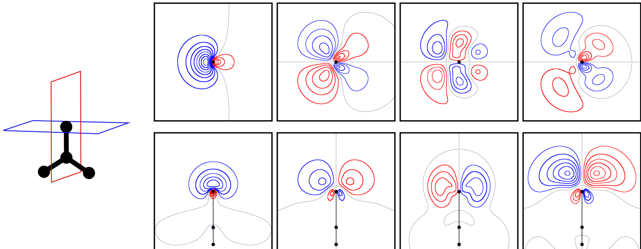
FIGURE 2. Examples of pOOs generated from the oxygen lone pair of the formaldehyde (left panels) by applying first-, second- and third order harmonics (second, third and last panels). The first row shows contour taken on the blue plane in the sketch molecule on the left, the second row shows contour taken on the red plane.
