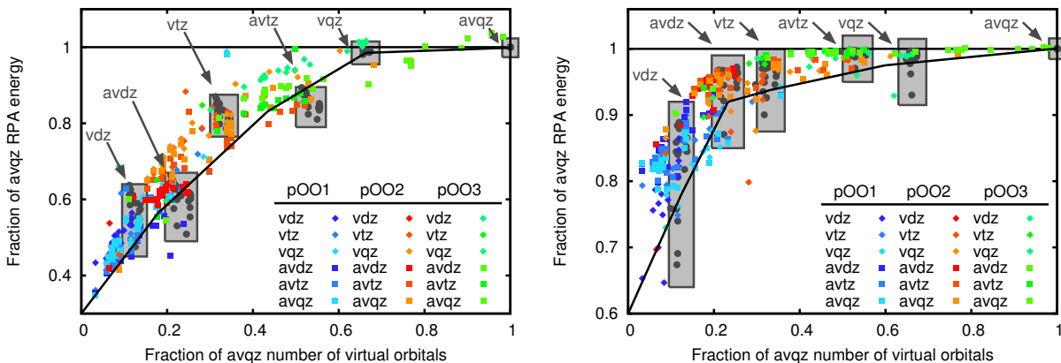
FIGURE 3. Results of calculations of the RPA correlation energies (left : full-range, right : long-range) of a small set of molecules. Each dot represents a result for one of those molecule, obtained with several different basis. The gray boxes gather the gray dots corresponding to reference results that are obtained with the unmodified cc-pVDZ, cc-pVTZ, aug-cc-pVTZ, cc-pVQZ and aug-cc-pVQZ basis sets (denoted as vdz, avdz, etc...). The color dots are the pOO results, with pOOs of first (second and third) order being in blue (red and green). Those pOOs can be obtained in the context of the different reference Dunning basis, hence the nuances of blue, red and green. The black line in both plots roughly connects the centers of the gray boxes.
