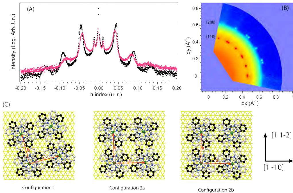
Figure 2: (A) : Scan along the [1\bar{1}0] direction of the reciprocal space of gold before (black dots) and after (pink dots) deposition of molecules. (B) : In-plane mesh ( l=0.05 Å) of the LuPc 2 /Au(111) after heating to 285°C. (C) : Representation of inequivalent domains of LuPc 2 on Au(111) lattice (colored in yellow), based on the experimentally determined 2D lattice and close packing of the LuPc molecules. The upper plateau LuPc 2 has been coloured in light grey for clarity. In-plane molecular distances are represented by plain line red arrows of a = 13.6 \pm 0.1 Å, b = 13.6 \pm 0.1 Å with an angle of 90 \pm 0.1^\circ between the two directions.
