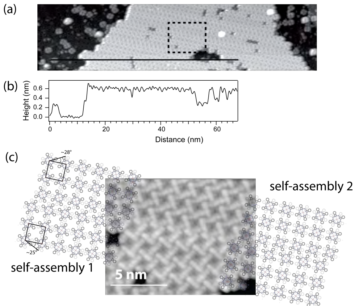
Figure 3: STM image recorded on \text{LuPc}_2 multilayer after annealing ( -2.6 V, 700 pA); (a) large scale image of area 100 nm \times 23.6 nm; (b) : height profile along the solid line drawn in the large scale image; (c) zoom region framed in the large scale image.
