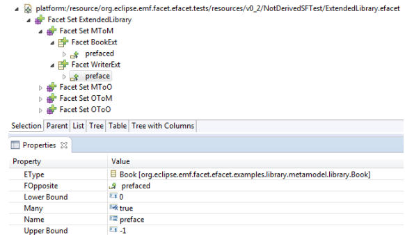
Figure 8: FacetSet definition example
