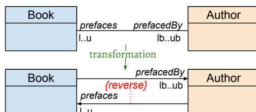
Figure 3: Bi-directional link example
