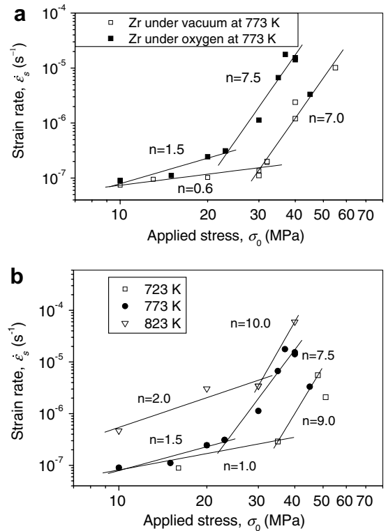
Fig. 4. Plot of the logarithm of strain rate, \dot{\epsilon}_s , against the logarithm of the applied stress, \sigma_0 , for zirconium: (a) at 773 K under vacuum and under oxygen; (b) at 723, 773 and 823 K under oxygen.
