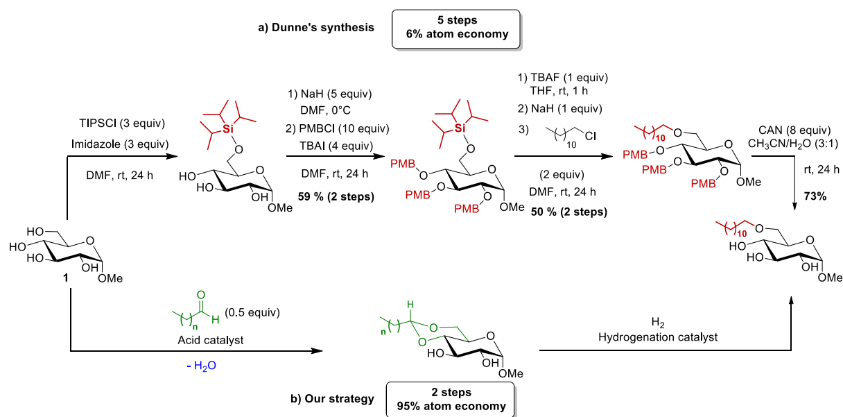
Scheme 1: Comparison of synthetic routes to access methyl 6-O-dodecyl- \alpha -D-glucopyranoside. TIPS = triisopropylsilyl, DMF = dimethylformamide, PMB = para -methoxybenzyl, TBAI = tetrabutylammonium iodide, TBAF = tetrabutylammonium fluoride, CAN = cerium ammonium nitrate.
