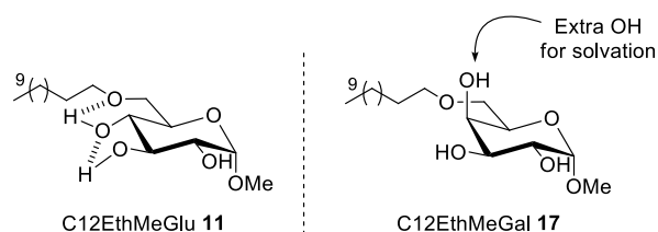
Figure 6. Model proposed to explain the polarity difference between C12EthMeGlu 11 and C12EthMeGal 17 (only one conformer showed).
