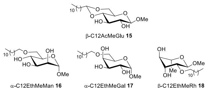
Figure 4. Range of acetal and ether derivatives obtained from acetalisation / hydrogenolysis sequence.
