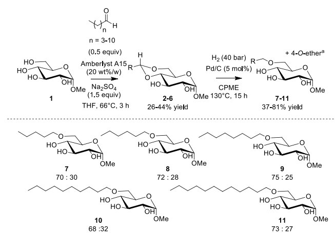
Scheme 2. Preparation of methyl \alpha -D-glucopyranoside ethers by acetalisation / hydrogenolysis sequence. a The 6-O : 4-O regioisomeric ratio was determined by GC chromatography after derivatization. CPME = cyclopentyl methyl ether.
