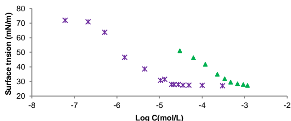
Figure 5. Surface tension of methyl \alpha -D-glucopyranoside ether vs methyl \alpha -D-galactopyranoside ether * C12EthMeGlu 11 , \blacktriangle C12EthMeGal 17 .
