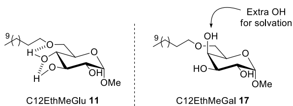
Figure 6. Model proposed to explain the polarity difference between C12EthMeGlu 11 and C12EthMeGal 17 (only one conformer showed).
