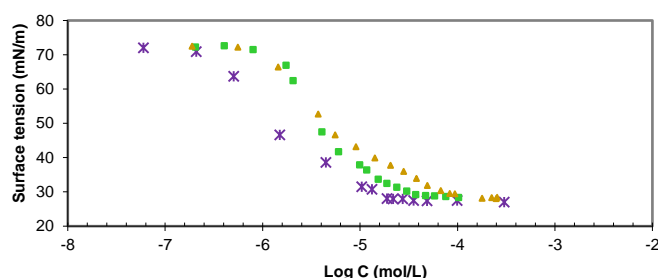
Figure 3. Surface tension vs concentration of methyl dodecyl- \alpha -D-glucopyranoside: \blacktriangle 4- O -isomer 11a , \blacksquare 6- O -isomer 11b , and \times a 73 : 27 mixture of 6- O - and 4- O -isomers 11 .
