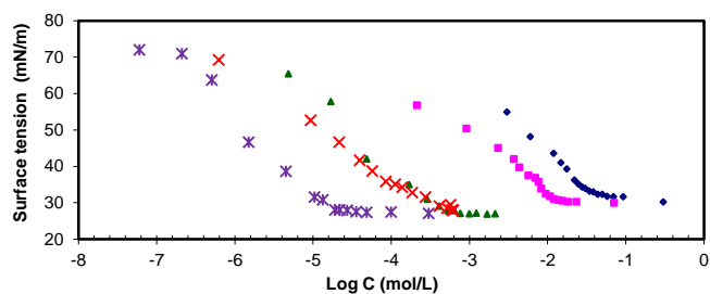
Figure 2. Surface tension vs concentration of methyl \alpha -D-glucopyranoside ethers (mixtures of regioisomers). \blacklozenge C5EthMeGlu 7 , \blacksquare C6EthMeGlu 8 , \blacktriangle C8EthMeGlu 9 , \times C10EthMeGlu 10 , \ast C12EthMeGlu 11 .
