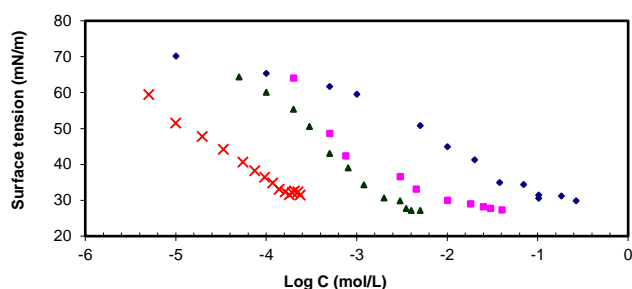
Figure 1. Surface tension vs concentration of methyl \alpha -D-glucopyranoside acetals. \blacklozenge C5AcMeGlu 2 , \blacksquare C6AcMeGlu 3 , \blacktriangle C8AcMeGlu 4 , \times C10AcMeGlu 5 .
