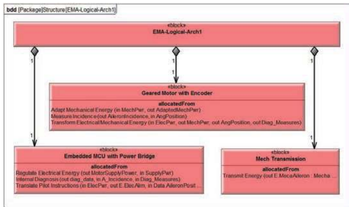
Fig. 8. System Structure
