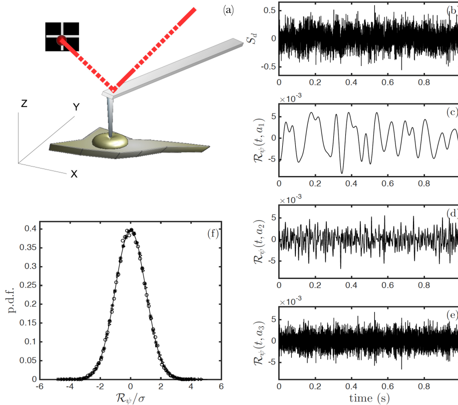
FIG. 7. (a) Sketch of the AFM principle. (b) Cantilever tip fluctuations S_d recorded from a normal C2C12 myoblast with a loading force of 1 nN. (c-e) Real part of the wavelet transform of S_d : \mathcal{R}_\psi(t, a) = \text{Re}[T_\psi[S_d](t, a)] for three different scale values a_i = f_0/f_i with f_1 = 10 Hz (o), f_2 = 10^2 Hz (*) and f_3 = 10^3 Hz ( \triangleright ). (f) P.d.fs of \mathcal{R}_\psi(\cdot, a)/\sigma(a) for the three scale values shown in (c-e), after rescaling by the corresponding standard deviation \sigma(a) . The solid line corresponds to the rescaled p.d.f. of S_d . The analyzing wavelet is a Morse wavelet of exponents \gamma = 1 , n = 1 (Eq. (13).)
