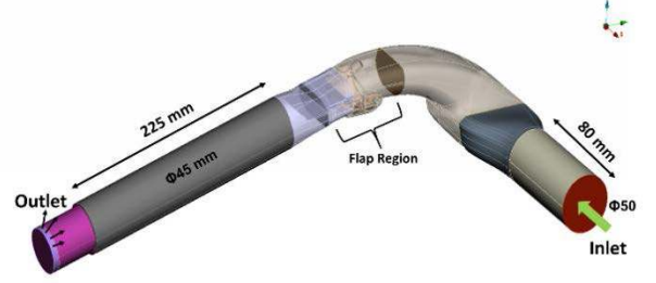
Fig. 3. Computational domain
