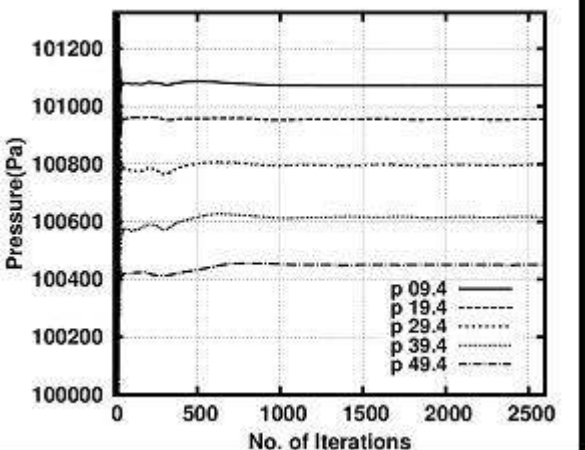
Fig. 5. Pressure at a point upstream of flap
