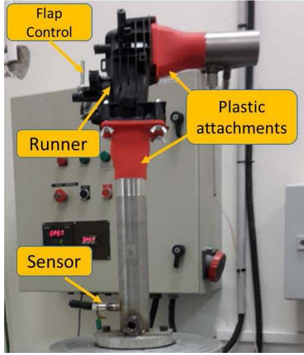
Fig. 2. Experimental setup
