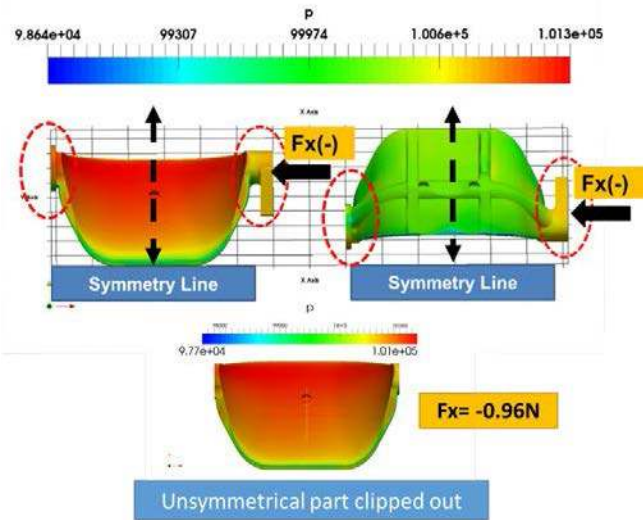
Fig. 9. Analysis of F_x on the flap
