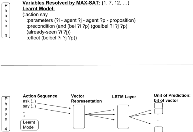
Figure 3: Illustration of Phases 3 and 4 of our approach. Phase 3 involves solving of the formulated constraints as a SAT problem to reconstruct the underlying model. Phase 4 involves using the previously learnt model to perform sequence labelling on the speech acts comprising the training data.
