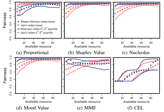
Fig. 4: Fairness w.r.t. the available resource (3 users, Zipf)
