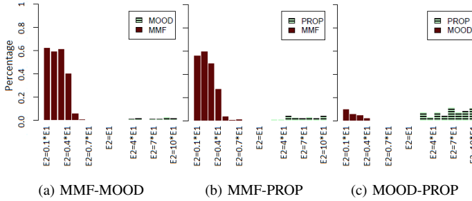
Fig. 9: Percentage of agglomerated equilibria in CASE 2.
