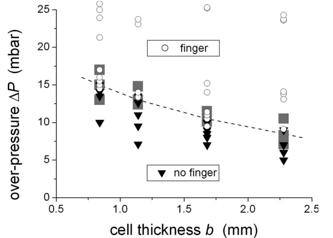
FIG. 3. Threshold pressure for the onset of grain mobilization and finger formation in the air-grain system. The gray squares correspond to the \Delta P at which fingering occurs for experiments where the injection pressure is gradually increased from zero. For the oil-grains system finger formation is observed for all tested \Delta P .
