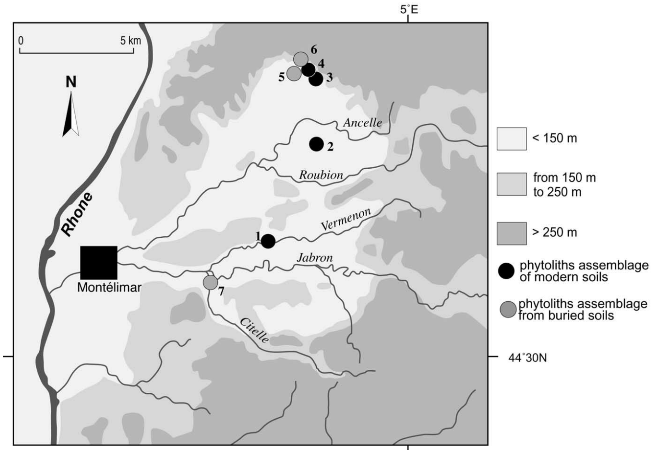
Fig. 2. The Valdaine Basin. Location of the main sampling sites: (1) river forest of Vermenon River at “les feuilles” site, (2) “Andran” forest on gravelly Würmian terrace, (3, 4) south slope of marly hills of Roynac, (5) prehistoric settlement of Roynac-le-Serre, (6) prehistoric settlement of Roynac-les-Roches, and (7) prehistoric settlement of Espeluche-Lalo.
