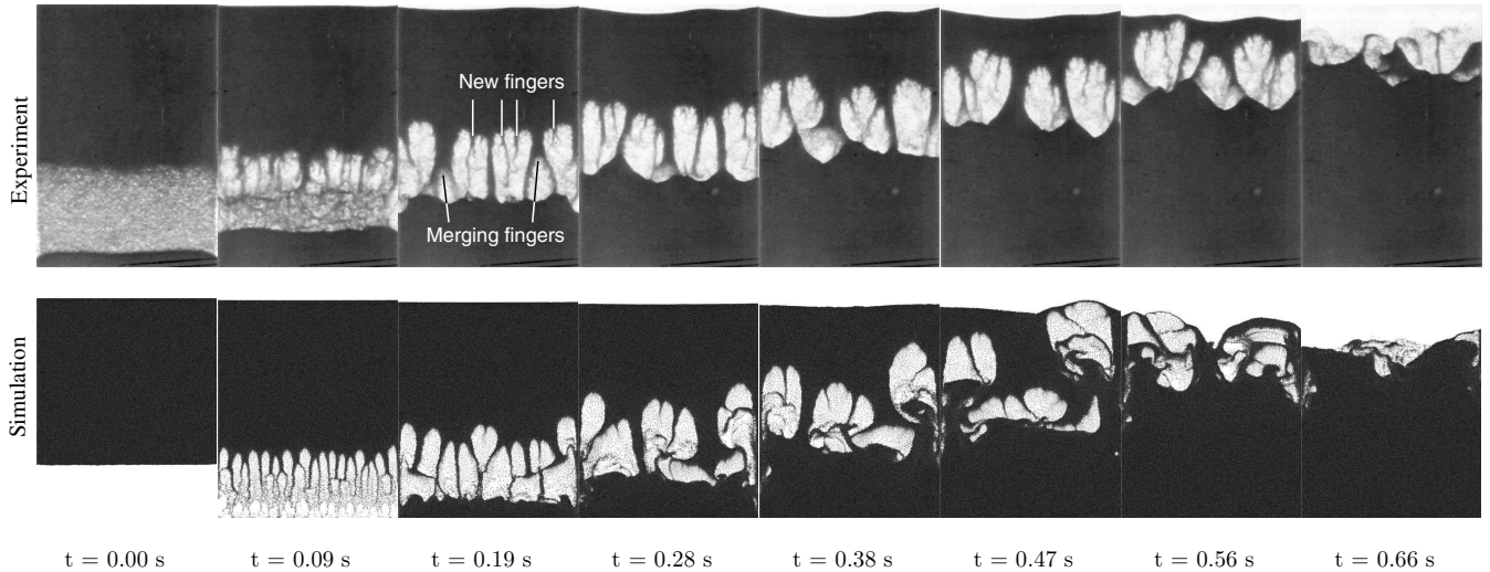
FIG. 4. Images from the experiment (top row) and simulation (bottom row) with polystyrene beads of 140 \mu\text{m} in diameter in a closed Hele-Shaw cell that is 56 \text{ mm} wide. The experimental cell is 86 \text{ mm} high and 1 \text{ mm} thick, while the numerical cell is 68 \text{ mm} high. The time of the snapshots is the time evolved since the cell reached the upright position. A restitution coefficient of 0.5 is used in the simulations.
