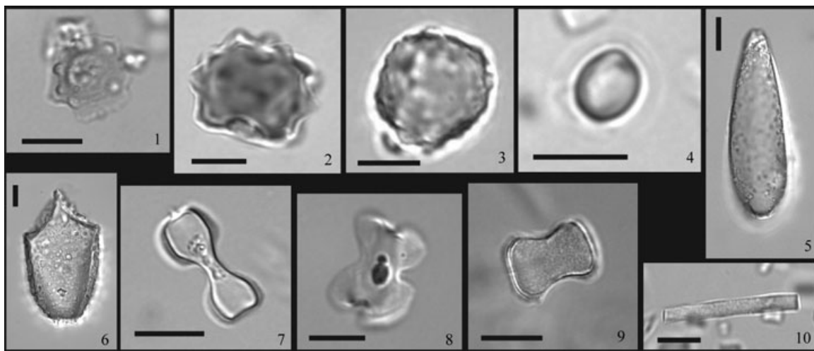
Figure 2 Microphotographs of representatives of the 10 types of identified phytoliths; Scale bar = 10 \mu\text{m} : (1) cone shaped type; (2) crenate spherical type; (3) rough spherical type; (4) smooth spherical type; (5) point-shaped; (6) fan-shaped type (also Fs); (7) dumbbell type; (8) cross type; (9) saddle type, (10) elongate type.
