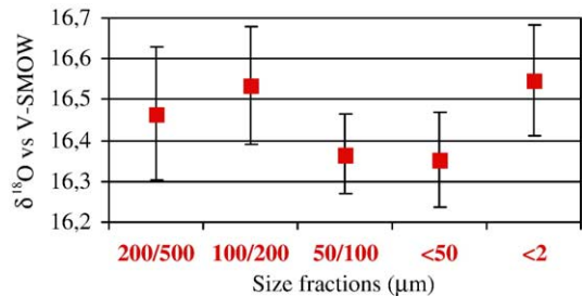
Fig. 1. Average \delta^{18}\text{O} values of several size fractions of the quartz lab standard “Boulangé” analyzed using Infra-red laser-heated fluorination technique. Average value: 16.46‰ vs. V-SMOW; Error bars give external precision calculated from replicate analyses: \pm 0.15\text{‰} ( \pm 1\sigma ); 76 analyses performed over 12 weeks. No \delta^{18}\text{O} trend with size is displayed which makes our laser heating protocol a success.
