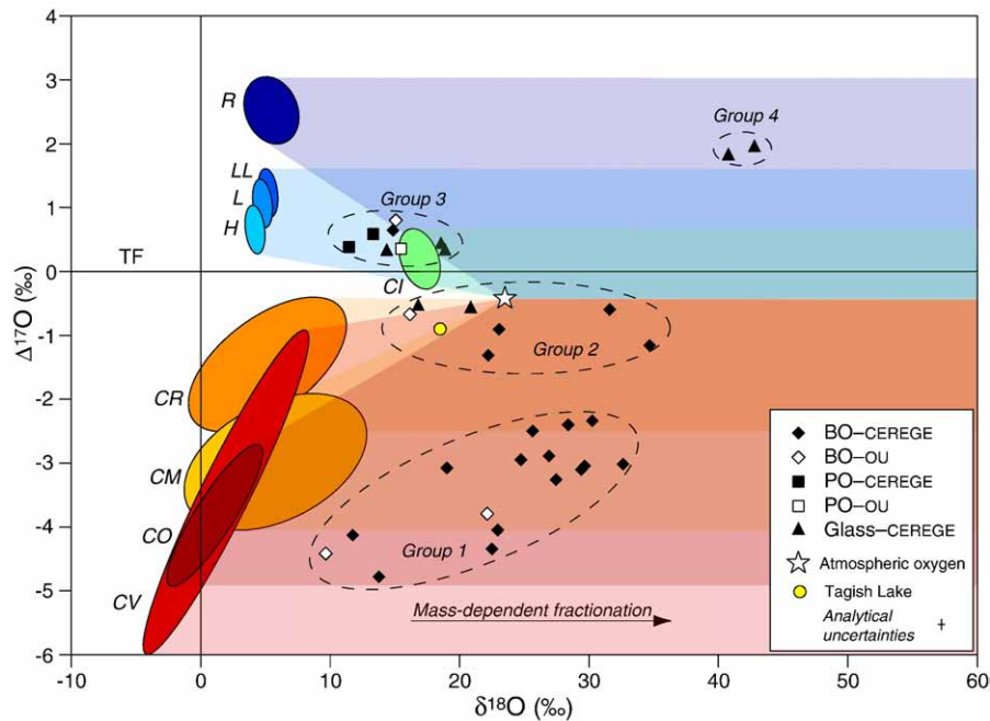
Fig. 4. Δ 17 O vs. δ 18 O values (in ‰ vs. V-SMOW) of individual cosmic spherules measured by IRMS (typical analytical uncertainties are represented: ±0.5‰ for δ 18 O, ±0.08‰ for Δ 17 O). Potential parent bodies are displayed by colored domains (Clayton et al., 1991; Clayton and Mayeda, 1999). The whole rock isotopic composition of Tagish Lake meteorite (Brown et al., 2000) is also represented. The range of possible values of Δ 17 O and δ 18 O for a micrometeorite from a given parent body is represented with a shaded area.
