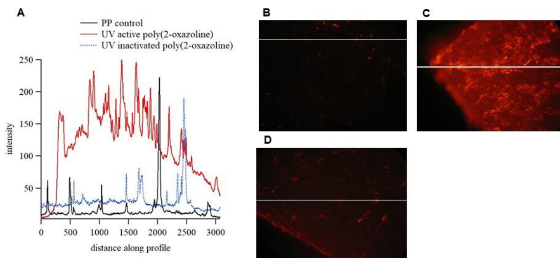
Figure S4. Line profiles of the individual red component along the specified path of all surface images shown (A). Fluorescence microscopy images of untreated PP surface (B), PP surface 5x irradiated for 20 min with UV active P[(\text{AzPhOx})_5\text{-}co\text{-(MeOx)}_{10}]\text{-}b\text{-(MeOx)}_{90} (C) and with UV inactivated P[(\text{AzPhOx})_5\text{-}co\text{-(MeOx)}_{10}]\text{-}b\text{-(MeOx)}_{90} (D).
