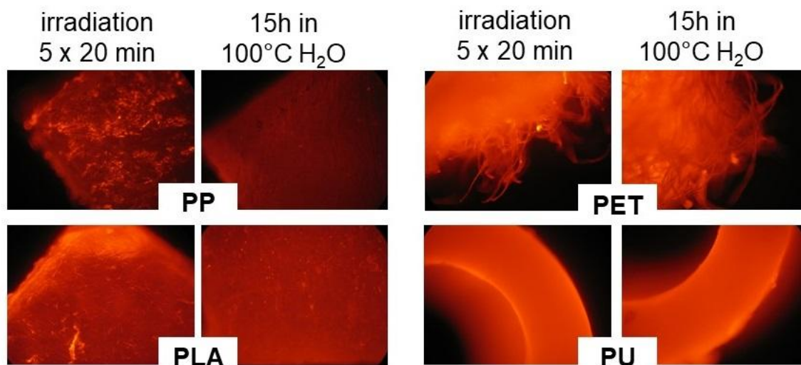
Figure 3. Visualization of the grafting process after five coating steps and its thermal stability in 100°C hot water by utilizing a fluorescent labeled P[(\text{AzPhOx})_5\text{-co-(MeOx)}_{10}]\text{-b-(MeOx)}_{90} copolymer on various materials.
