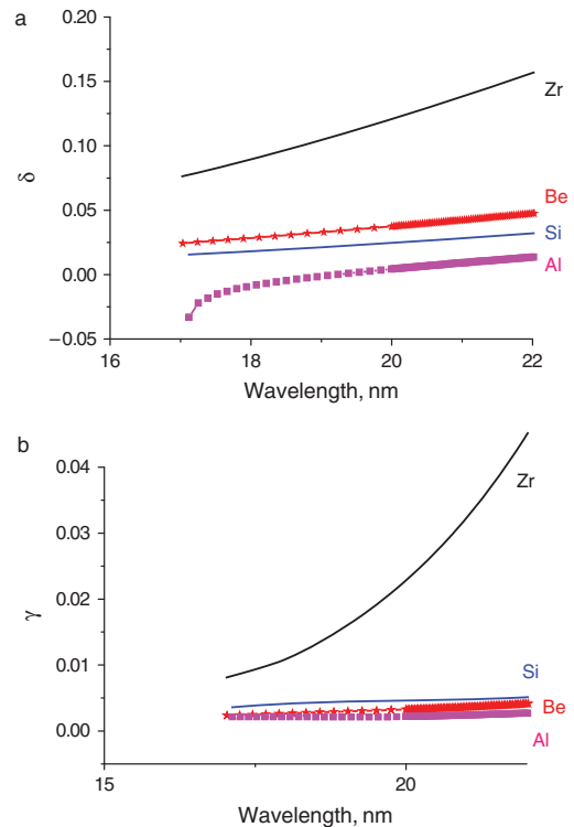
Figure 4. Dispersive additives to the real (a) and imaginary (b) parts of the refractive index for Zr, Si, Al, and Be.
