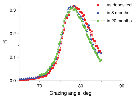
Figure 7. Angular dependencies of the reflection coefficient of the Be/Si/Al mirror at a wavelength of 30.4 nm immediately after the deposition, after 8 months and after 20 months after the deposition.
