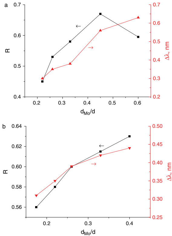
Figure 3. Dependencies of the peak values of the reflection coefficients R and their spectral widths \Delta\lambda on \beta_{Mo} . (a) Corresponds to Mo/Si, (b) to Mo/Be MLM.
