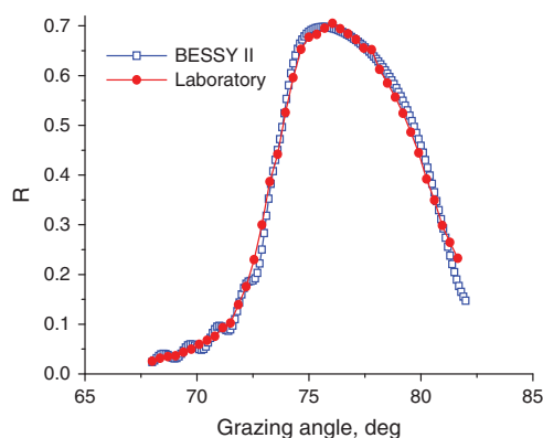
Figure 1. Angular dependencies of the reflection coefficient of the Mo/Be mirror, measured on a laboratory reflectometer 22 and on BESSY-II. 24 The wavelength is 11.34 nm.
