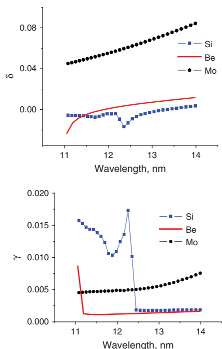
Figure 2. Dispersive additions to the refractive indices ( n = 1 - \delta + i\gamma ) of molybdenum, silicon and beryllium in the 11–14 nm region.
