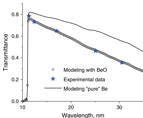
Figure 8. Spectral dependence of the transmittance of a 160 nm thick Be film. The asterisks represent the experimental data measured on the characteristic lines BeK \alpha (11.4 nm), SiL \alpha (13.5 nm), AlL \alpha (17.1 nm), MgK \alpha (25.0 nm) and HeII (30.4 nm). The calculated dependence (scatter line) takes into account the presence of beryllium oxide on the film’s surfaces. The fitting gives 3.5 nm of BeO on each side. Other calculated dependence (solid line) show of the transmittance of a 160 nm thick Be film.
