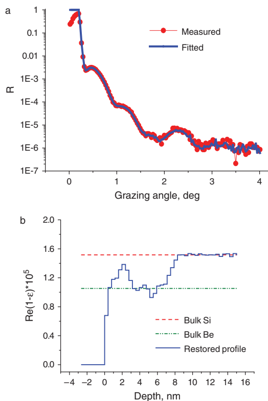
Figure 9. (a) Reflectivity of a Be film sputtered onto a Si substrate at \lambda = 0.154 nm. (b) The polarizability profile of the film.
