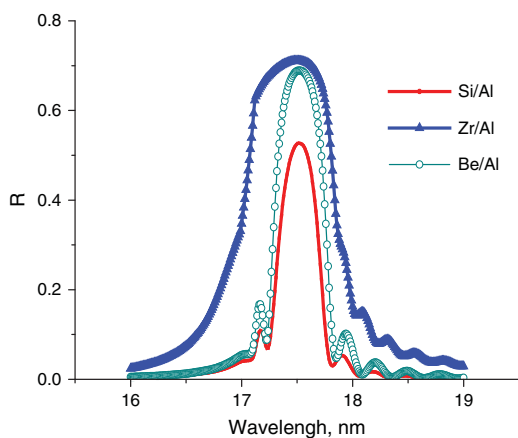
Figure 5. Calculated spectral dependencies of the reflection coefficients of Zr/Al, Si/Al and Be/Al MLM at normal incidence. The calculations are made for “ideal” structures with a tabular density of materials and zero roughness, the composition of which is optimized for a maximum of the reflection coefficient.
