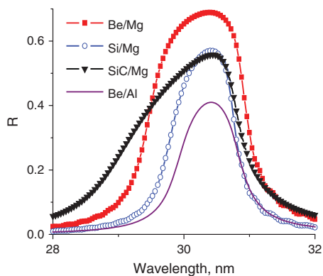
Figure 6. Calculated spectral dependencies of the reflection coefficients of the most optimal MLM among magnesium-based mirrors and the Be/Al structure.
